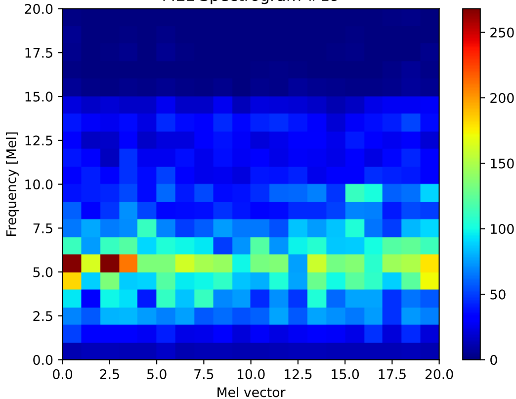
MEL Spectrogram #19
